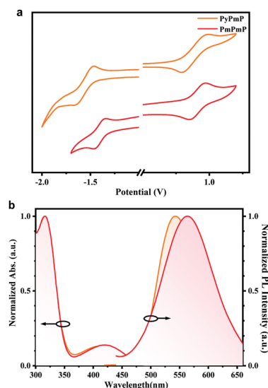
Fig. 2 (a) Cyclic voltammograms of PyPmP and PmPmP measured in DMF, and (b) their normalized absorption and emission spectra in dilute toluene at ambient temperature. Molecular structures of PyPmP and PmPmP and their simulated HOMO/LUMO energy levels and spatial distributions. The isovalue is 0.02.
