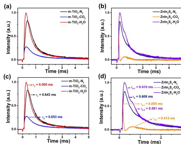
Fig. 6 (a, b) Comparison of the in situ TPV curves of \text{m-TiO}_2 and \text{ZnIn}_2\text{S}_4 under \text{N}_2 -saturated MeCN, \text{CO}_2 -saturated MeCN, and 0.5 vol% \text{H}_2\text{O} /MeCN (v/v). (c, d) The corresponding attenuation constants ( \tau ) of the charge recombination process.
