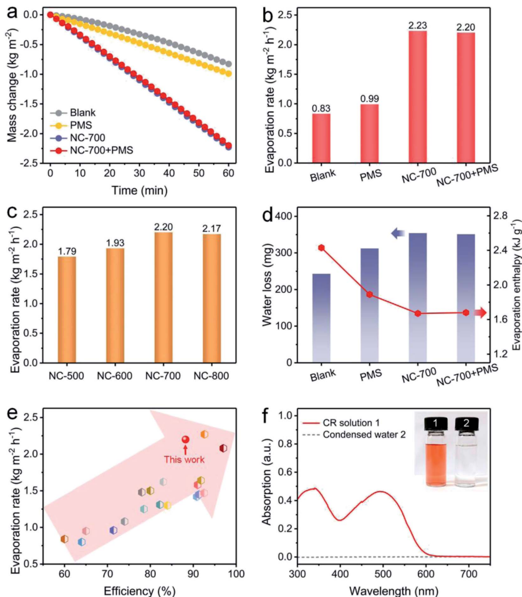
Fig. 6 (a) Water mass change and (b) evaporation rate under diverse conditions: blank (100 ppm of the CR solution under 1 kW \text{m}^{-2} irradiation), PMS (adding cotton and 0.15 g \text{L}^{-1} PMS), NC-700 (adding the NC-700 evaporator), and NC-700 + PMS (adding the NC-700 evaporator and 0.15 g \text{L}^{-1} PMS). (c) Evaporation rate using the NC-x evaporator under 1 sun irradiation. (d) Water loss of the CR solution in darkness and the evaporation enthalpy. (e) Comparison of the performance of the NC-700 evaporator with some previous works. (f) UV-Vis curves of the CR solution and condensed water.
