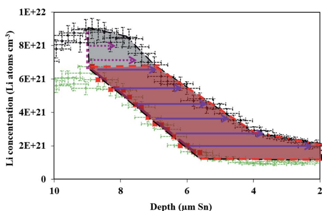
Fig. 6 The black shaded area between the spectra represents the total Li content added to the electrode between 10 h and 20 h of the 600 mV hold. The red shaded area represents the portion of that Li added which diffuses into the electrode down a pre-existing concentration gradient (red squares). When calculating the flux for Fick's 1st law only the Li content which diffuses down a gradient (purple arrows) is included. The Li added to the electrode at the interface (pink dotted line) for which there is no previous gradient (pink dotted arrows) is not included in the flux calculation.
