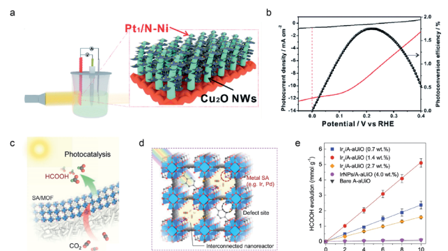
Fig. 6 (a) Schematic illustration and (b) PEC performance of \text{Pt}_1/\text{N-Ni}/\text{Cu}_2\text{O} NWs for water reduction. 24 Reproduced with permission from ref. 24. Copyright 2021, The Royal Society of Chemistry. The scheme of (c) MOF membrane and (d) MOF structures with single metal atoms for photocatalytic \text{CO}_2 reduction. (e) Time course of HCOOH evolution on A-aUiO, \text{Ir}_1/\text{A-aUiO} , \text{Ir}_x/\text{A-aUiO} and IrNPs/A-aUiO catalysts. 74 Reproduced with permission from ref. 74. Copyright 2021, Springer Nature.
