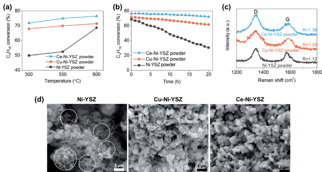
Fig. 1 The steam reforming of butane using powder catalysts. (a) Butane conversion levels from 500 to 600 °C using various Ni-YSZ powder samples at an SCR of 3. (b) Long-term testing of the steam reforming of butane at 600 °C with an SCR of 3 for 20 h. (c) Raman spectra and (d) SEM images of various Ni-YSZ powder samples after 20 h of the steam reforming of butane.
