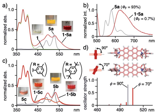
Fig. 5 (a) UV-visible spectra and photographs (5 : 1 water/AN, r.t.) of 1·5a, 1, and 5a (in CH_2Cl_2 ) and (b) their fluorescence spectra ( \lambda_{ex} = 500 nm) except for 1. (c) UV-visible spectra (5 : 1 water/AN, r.t.) of 1·5b, 1·5c, 5b (in CH_2Cl_2 ) and 5c (in DMSO). (d) Optimized structures of 5a with \phi = 90^\circ and 70^\circ and their predicted, electronic absorption bands. 15
