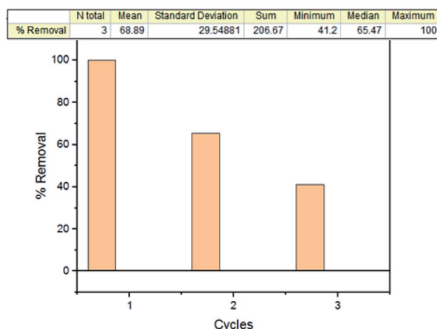
Fig. 15 % (TP) removal for 0.3 g dosage, 30 \text{mg-P L}^{-1} initial concentration, \text{pH} = 2 , and time of 105 minutes for each cycle.
