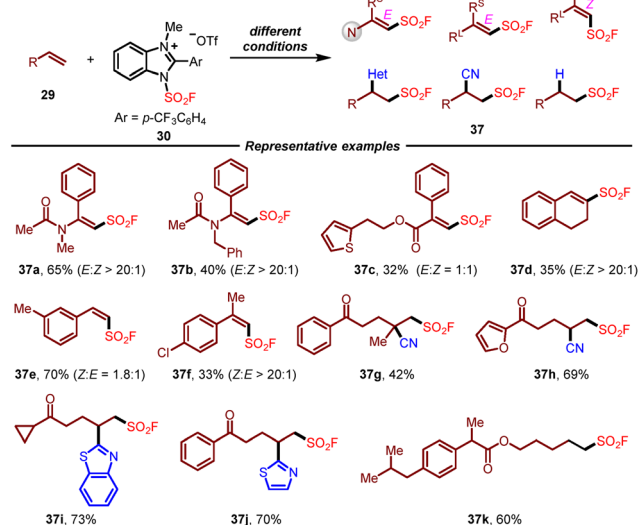
Scheme 6 Synthesis of alkenyl and alkyl sulfonyl fluorides with a benzoimidazolium-based fluorosulfonyl radical precursor.
