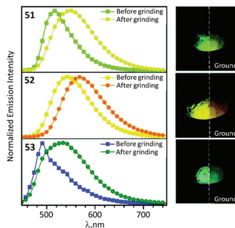
Fig. 11 Solid-state emission spectra of 51–53 before and after grinding using \lambda_{\text{ext}} = 365 nm; photographs taken under UV lamp illumination ( \lambda_{\text{ext}} = 365 nm). Adapted with permission from ref. 49. Copyright (2020) The Royal Society of Chemistry.
