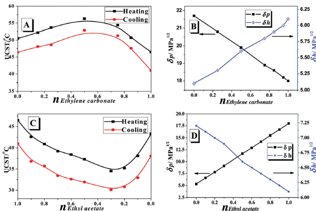
Fig. 49 (A) UCST and (B) and \delta p and \delta h of TRPSis in acetonitrile/ethylene carbonate mixed solvents as a function of the ethylene carbonate content; (C) UCST and (D) \delta p and \delta h of TRPSis in acetonitrile/ethyl acetate mixed solvents as a function of the ethyl acetate content. Reproduced from ref. 96 Copyright 2017 Royal Society of Chemistry and the Centre National de la Recherche Scientifique.
