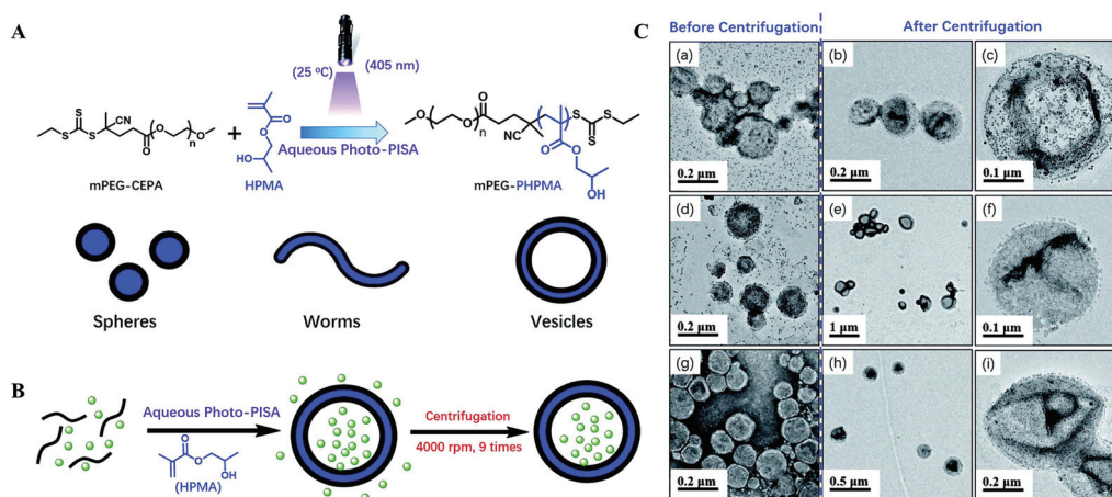
Fig. 8 (A and B) Schematic illustration of the preparation of hybrid vesicles loaded with silica nanoparticles via aqueous photo-PISA of HPMA. (C) TEM images of unpurified and purified mPEG 113 -PPHMA 365 hybrid vesicles prepared via aqueous photo-PISA of HPMA by adding different amounts of silica sol. Reproduced with permission from ref. 157. Copyright © 2017, Royal Society of Chemistry.
