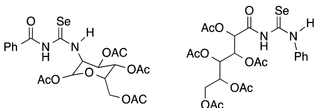
Fig. 2 Acylselenoureas derived from carbohydrates.
