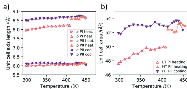
Fig. 5 a) Lattice constants a and b during heating ( \blacktriangleright , \triangle ) and cooling ( \blacktriangleleft , \nabla ). The filled triangles denote the high temperature polymorph II. It can be seen that the change in length is stronger for the b -axis in both polymorphs upon heating and cooling. b) The in-plane unit cell areas of both polymorphs plotted against the temperature. The filled in triangles denote polymorph II.
