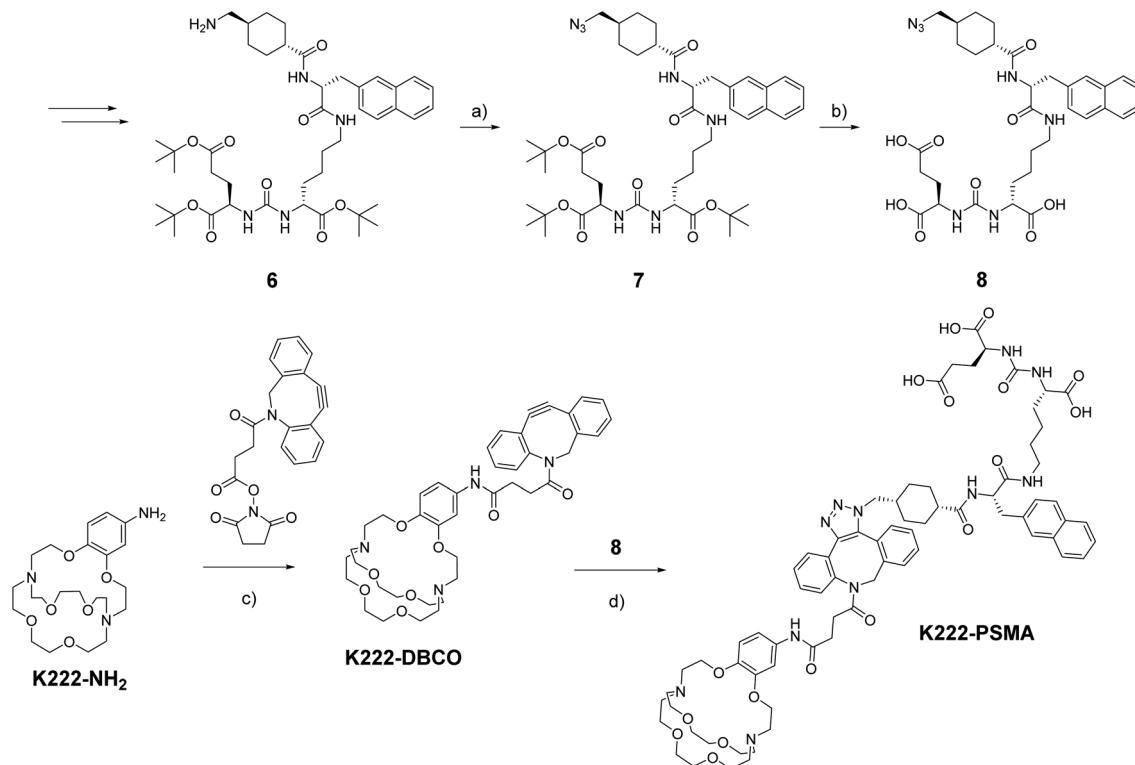
Scheme 2 Synthetic route towards K222-DBCO and K222-PSMA Reaction conditions: (a) FSO 2 N 3 , 3 M KHCO 3 , MTBE/DMF/H 2 O, r.t., 5 min; (b) TFA, DCM (1 : 2), r.t., 3 h; (c) DBCO-NHS, DMF, r.t., overnight; (d) 8 , DMF/MeOH (1 : 1), r.t., overnight.
