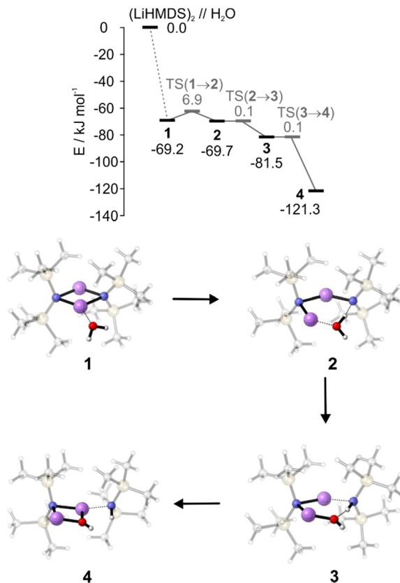
Fig. 5 Potential energy surface (PES) of the reaction of (\text{LiHMDS})_2 with \text{H}_2\text{O} and minima 1–4 . The PES energies of the minima are given relative to non-interacting (\text{LiHMDS})_2 and \text{H}_2\text{O} . Energies of transition states are given relative to the starting material. All calculations are carried out at the B3LYP-D3/def2-TZVP level of theory (without zero-point energy correction).
