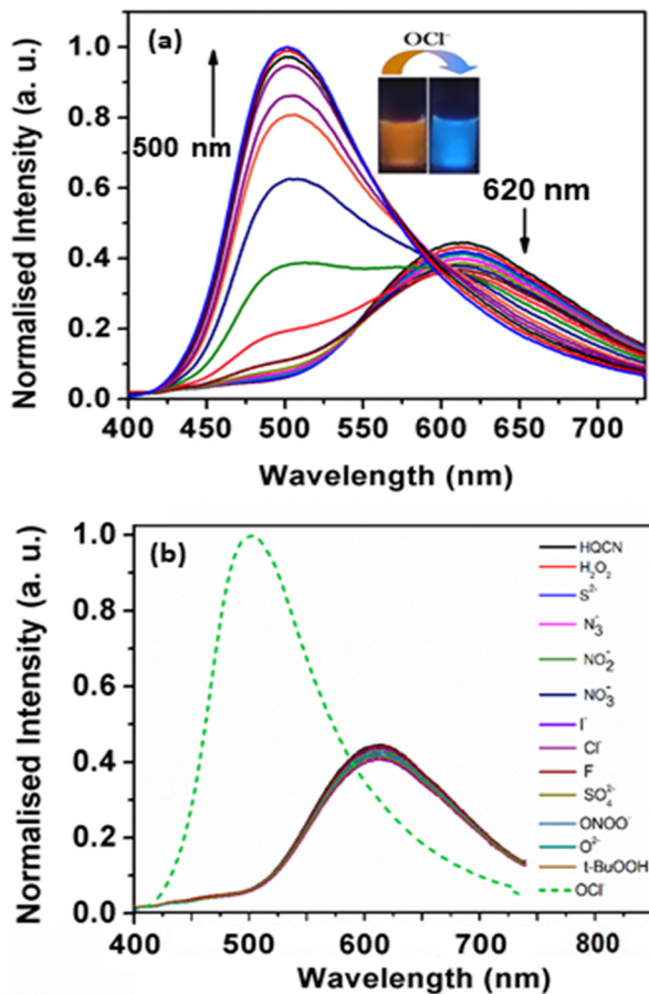
Fig. 4 (a) Fluorescence emission of HQCN ( 10 \mu\text{M} in \text{CH}_3\text{OH}-\text{H}_2\text{O} ; 1/4, v/v in the presence of HEPES buffer (10 mM) solution at \text{pH} = 7.2 ) upon the gradual addition of \text{OCl}^- (0 to 5 equivalents). Ratiometric spectra of HQCN were observed after the addition of \text{OCl}^- , where the \lambda excitation was 370 nm. The fluorescence emission peak at 620 nm gradually decreased and the peak at 500 nm gradually increased after the addition of \text{OCl}^- . Inset shows the visible emission of HQCN in the absence and presence of 2 equivalents of \text{HOCl} upon irradiation under UV light. (b) Fluorescence emission spectra of HQCN ( 10 \mu\text{M} in \text{CH}_3\text{OH}-\text{H}_2\text{O} ; 1/4, v/v in the presence of HEPES buffer (10 mM) solution at \text{pH} = 7.2 ) upon addition of different guest analytes (0 to 5 equivalents). Apart from \text{OCl}^- , no significant change was observed for other guest analytes.
