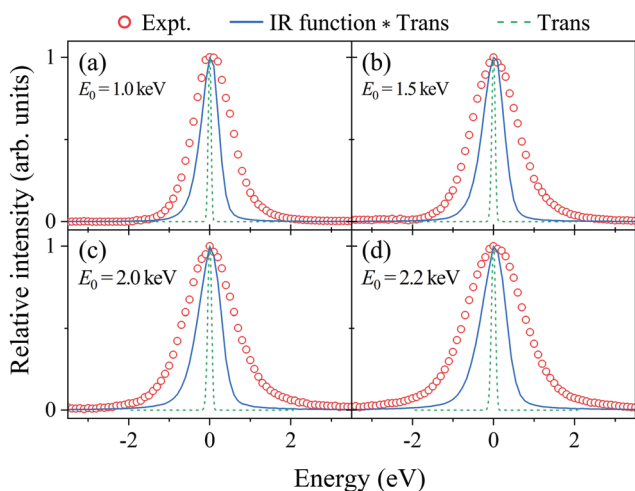
Fig. 3 Energy spectra of H 2 obtained at E_0 = (a) 1.0, (b) 1.5, (c) 2.0, and (d) 2.2 keV, respectively. The solid lines are the associated practical instrumental response (IR function \times Trans). The dashed lines are the calculated Doppler broadening due to molecular translational motion.
