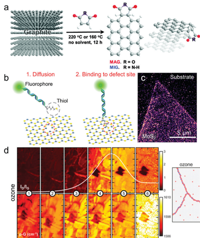
Fig. 2 (a) Schematic drawing of edge functionalization and delamination of graphite edge by Diels–Alder reaction with maleimide (reprinted with permission from ref. 131 Copyright 2014 Chemical Communications). (b) Schematic drawing of selective chemisorption of a thiol group to S vacancy site of MoS 2 . (c) Fluorescent microscope image of fluorophore attached to MoS 2 vacancy site (reprinted with permission from ref. 136 Copyright 2021 ACS Nano). (d) (left) G peak position Raman map of ozone functionalized graphene near grain boundary, for six different oxidation steps. (right) Schematic of defect (red) accumulated at grain boundary (reprinted with permission from ref. 156 Copyright 2015 2D Mater. ).
