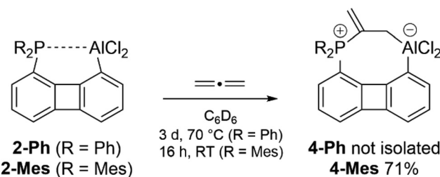
Scheme 4 Activation of propadiene by 2-R .
