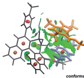
Fig. 4 (A) E_O'' and E_{N,I}''' shown here are the computed lowest-energy conformations of the ternary complex \text{CF}_3\text{-DSI } 2b/E\text{-}5b/3c . E_O'' accommodates all the experimental NOE and HOESY connections (key NOEs/HOEs are shown in the structures computed at TPSS-D3(BJ)/def2-SVP/SMD). Table 1 shows \Delta G_{(\text{DCM},180\text{ K})} for the principal conformations (free energy corrections and solvation corrections at the geometry optimization level of theory were added to the single-point total electronic energies). Table 2 illustrates the relative stabilities \Delta G_{(\text{DCM},180\text{ K})} of the conformationally refined structures. (B) Binding of the Hantzsch ester occurs at the oxygen atoms as evidenced by electrostatic potential map of the binary E_N and ternary E_O complexes. (C) Noncovalent interaction plot of complex E_O'' , suggesting that dispersion contributes significantly to stabilization of the ternary complex. (D) Dispersion interaction density plot confirms the importance of dispersion within complex E_O'' (computed at DLPNO-CCSD(T)/def2-TZVP level of theory).
