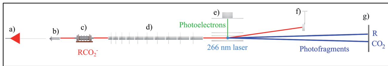
Fig. 1 Schematic of the high beam energy PPC spectrometer depicting the (a) ESI source, (b) octopole ion guide, (c) hexapole accumulation trap, (d) LINAC, (e) electron detector, (f) undetached ion deflector and (g) neutral detector. 24 The 4.66 eV DPD of \text{RCO}_2^- is also shown.
