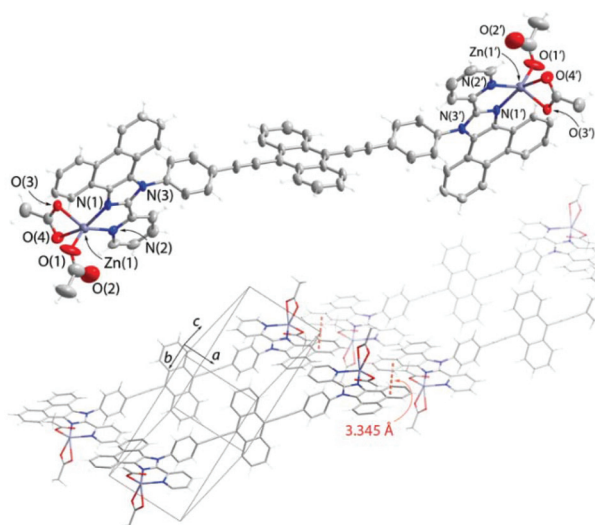
Fig. 12 Molecular view and packing fragment of 3OAc y . Crystallization solvent was disordered and omitted from the refinement model. The intermolecular \pi - \pi distances were measured between the planes of the phenanthrene motifs. Symmetry transformations used to generate equivalent atoms ( ' ): -x, 1 - y, -z . Thermal ellipsoids are shown at the 50% probability level.
