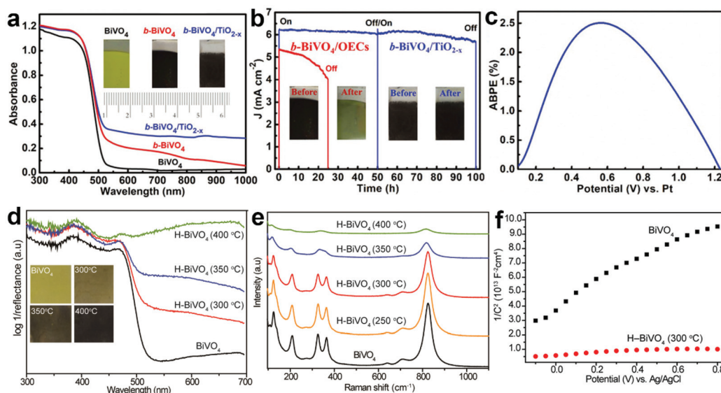
Fig. 10 (a) UV-vis absorption spectra of the \text{BiVO}_4 , b\text{-BiVO}_4 , and b\text{-BiVO}_4/\text{TiO}_{2-x} photoanodes. Inset: digital images of the \text{BiVO}_4 , b\text{-BiVO}_4 , and b\text{-BiVO}_4/\text{TiO}_{2-x} photoanodes. (b) Photocurrent density versus time plots of the b\text{-BiVO}_4/\text{TiO}_{2-x} and b\text{-BiVO}_4/\text{FeOOH}/\text{NiOOH} photoanodes for PEC water splitting at 1.23 V versus RHE. (c) ABPE curve of the b\text{-BiVO}_4/\text{TiO}_{2-x} photoanode obtained in a two-electrode cell for PEC water splitting. Reproduced from ref. 148 with permission. Copyright 2019, Wiley-VCH. (d) UV-vis absorption spectra of the air-annealed \text{BiVO}_4 film and \text{H-BiVO}_4 films hydrogen treated at 300, 350, and 400 °C. Inset: digital images of the air-annealed \text{BiVO}_4 film and \text{H-BiVO}_4 films. (e) Raman spectra of the air-annealed \text{BiVO}_4 film and \text{H-BiVO}_4 films hydrogen treated at 300, 350, and 400 °C. (f) Mott–Schottky plots of \text{BiVO}_4 and \text{H-BiVO}_4 (300 °C) in the dark with a frequency of 10 kHz. Reproduced from ref. 147 with permission. Copyright 2013, American Chemical Society.
