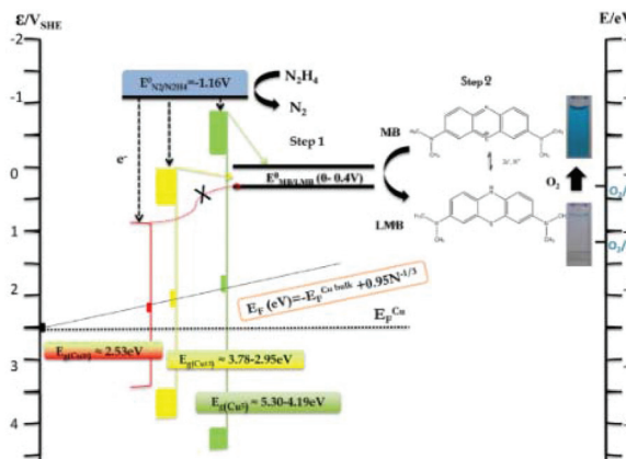
Fig. 36 Schematic energy diagram showing the catalytic activity of different CuNCs used for MB reduction by N 2 H 4 . Reprinted with permission from ref. 423. Copyright 2012 American Chemical Society.
