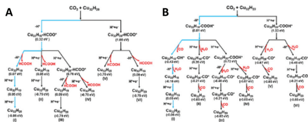
Scheme 9 Theoretical reaction schemes for CO 2 electroreduction on [Cu 32 H 20 {S 2 P(O i Pr) 2 }] 12 to form (A) HCOOH and (B) CO via six different pathways as described in ref. 188 (Reprinted with permission, Copyright 2017 American Chemical Society). The calculated free energy difference ( \Delta G ) for each elementary step is shown under each intermediate state. The most favourable reaction pathway is highlighted in blue.
