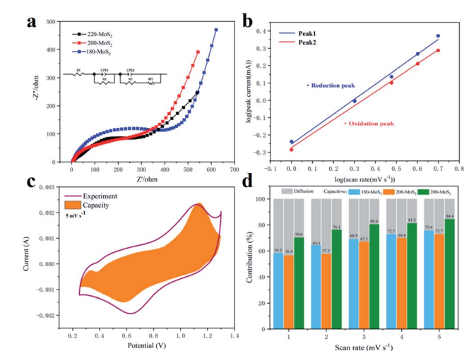
Fig. 7 (a) Electrochemical impedance spectroscopy of MoS 2 at different temperatures (inset is the equivalent circuit for fittings of the Nyquist plots of MoS 2 ), (b) \log(i) and \log(v) curves of two peaks corresponding to the CV curves (200-MoS 2 ), (c) capacitive contribution (orange) of 5 mV s -1 , (d) capacitive and diffusion-controlled contribution ratios at multiple scan rates of MoS 2 .
