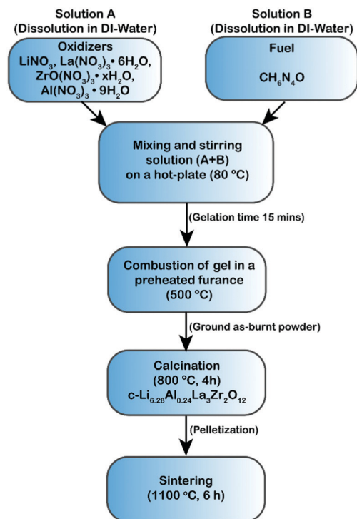
Fig. 1 Schematic representation of the combustion synthesis process for Al-LLZO.
