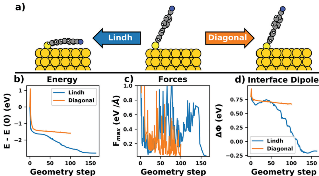
Fig. 20 Geometries of a cyano-biphenylthiole molecule on Au(111), calculated in a 5 \times 2\sqrt{3} unit cell with FHI-aims using the PBE+vdW surf method and a 3 \times 2 \times 1 \Gamma -centered k -point grid. A three-layer metal slab was used. All atoms of the molecule and the topmost layer of the slab were allowed to relax until the remaining forces on all atoms fell below 0.01 \text{ eV \AA}^{-1} . The calculations can be found on the NOMAD database. [https://dx.doi.org/10.17172/NOMAD/2020.12.07-9]. (a) Shows the starting geometry (center) and the final result after the optimization using a diagonal guess for the Hesse matrix (right) or using a Lindh guess (left). (b) Shows the evolution of the total energy relative to the energy of the starting point, for the two geometry optimizations. (c) Shows the remaining maximum force component F at each iteration step, (d) gives the interface dipole \Delta\phi .
