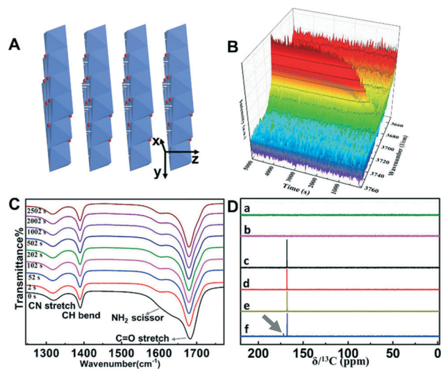
Fig. 4 (A) Atomic structure of \text{Co}(\text{OH})_2 , \text{Fe}(\text{OH})_2 , \text{Mn}(\text{OH})_2 , \text{Zn}(\text{OH})_2 , \text{Cu}(\text{OH})_2 \cdot \text{H}_2\text{O} and \text{Mg}(\text{OH})_2 . (B) Evolution of the typical O-H stretching mode of the Mg-OH groups over time. (C) FTIR spectra of the reaction process after introducing \text{NH}_3 into the formamide aqueous solution containing \text{MgCl}_2 in the 1000–2000 \text{cm}^{-1} region. (D) ^{13}\text{C} NMR spectra of (a) pure water after introducing \text{NH}_3 , (b) aqueous solution containing \text{MgCl}_2 after introducing \text{NH}_3 , (c) pure formamide aqueous solution, (d) formamide aqueous solution containing \text{MgCl}_2 , (e) formamide aqueous solution after introducing \text{NH}_3 without \text{MgCl}_2 and (f) formamide aqueous solution containing \text{MgCl}_2 after introducing \text{NH}_3 .
