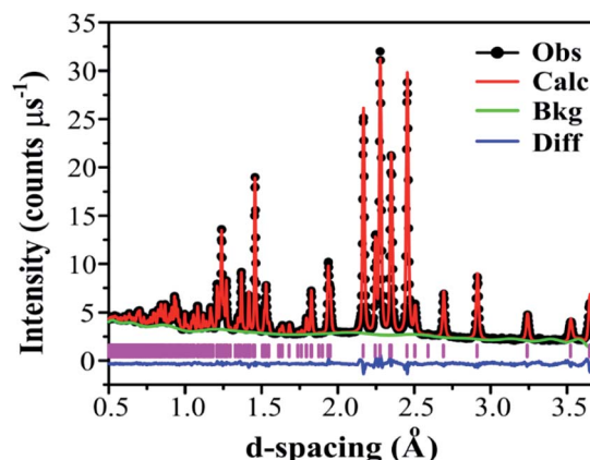
Fig. 5 Fitted neutron diffraction histogram for \text{Ba}_3\text{VWO}_{8.5} at ambient temperature. The TOF neutron diffraction data from the 90^\circ bank detector of the Polaris diffractometer is shown. Black dots indicate the observed data, the red line the Rietveld fit, the blue line indicates the difference between the observed and the calculated patterns, the green line the background function, and the pink vertical bars the reflection positions.
