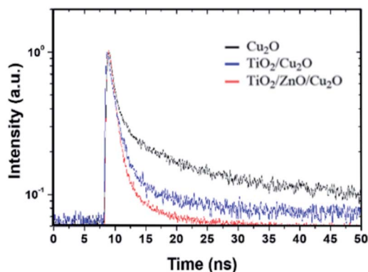
Fig. 5 Time-resolved PL spectra acquired with an excitation wavelength of 405 nm for the prepared Cu 2 O (black), TiO 2 /Cu 2 O (blue) and TiO 2 /ZnO/Cu 2 O (red) photoelectrodes.
