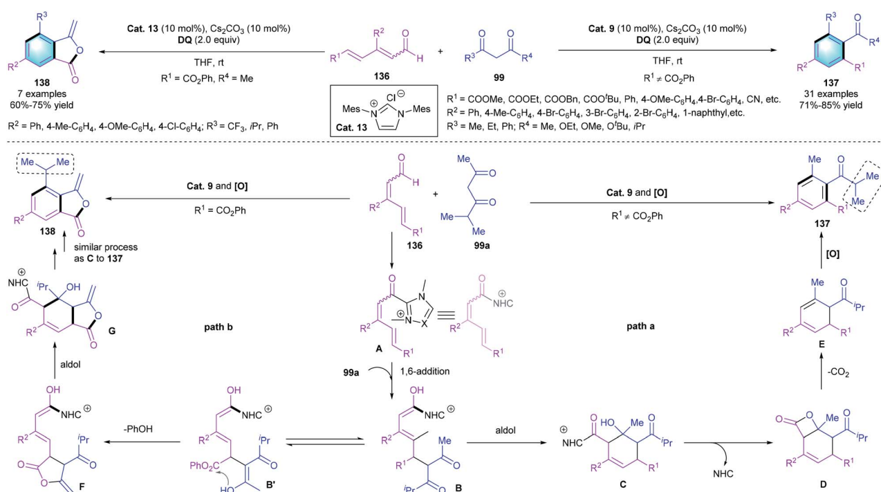
Scheme 39 NHC-catalyzed and substrate-controlled [4 + 2] benzannulation to synthesize tetra-substituted arenes or 3-ylideneephthalides.
