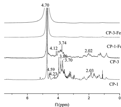
Fig. 5 1 H NMR spectra of polysaccharides and polysaccharide-iron(III) chelates.
