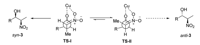
Scheme 11 You's asymmetric diastereoselective Henry reaction.
