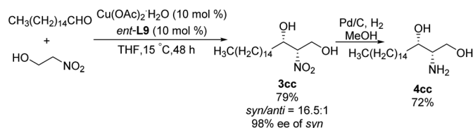
Scheme 18 Synthesis of safigol.
