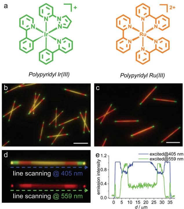
Fig. 3 (a) Chemical structures of the Ir donor and Ru acceptor. The similar molecular structures ensure the collaborative assembly of the two compounds. (b and c) Fluorescence microscopy images of hetero-junction nanorods doped with (b) 1%, and (c) 2% Ru acceptor under UV irradiation, showing multiple-color emissions. Scale bars are 20 \mu\text{m} . (d) Line scanning along a single nanorod using a confocal laser scanning microscope equipped with 405 and 559 nm lasers. (e) The corresponding plots of the microarea emission intensity as a function of the distance d along the rod axis. Reproduced with permission from ref. 23. Copyright 2018, American Chemical Society.
