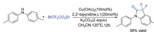
Scheme 101 The copper-catalyzed annulation of N -substituted anilines.
