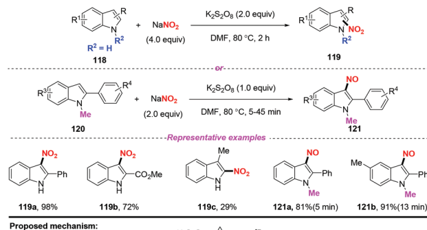
Scheme 44 Ionic liquid as nitrating reagent for the nitration of arylboronic acids, \alpha,\beta -unsaturated acids and benzoic acid derivatives.
