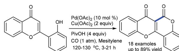
Scheme 111 Carbonylation of 2-phenolchromone.
