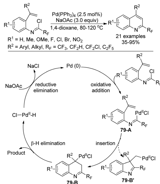
Scheme 79 Synthesis of 2-fluoroalkyl quinolines.
