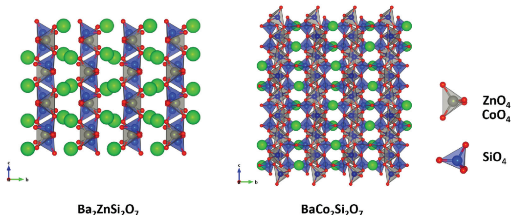
Fig. 7 Crystal structure of Ba 2 ZnSi 2 O 7 and BaCo 2 Si 2 O 7 .
