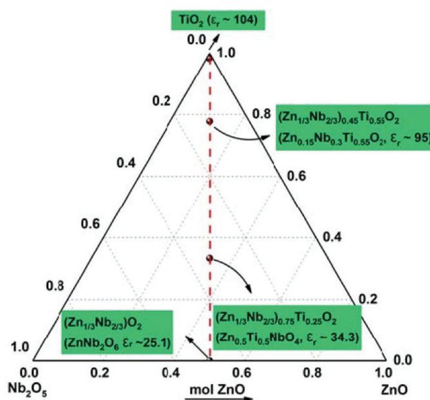
Fig. 39 Ternary ZnO–TiO 2 –Nb 2 O 5 systems.
