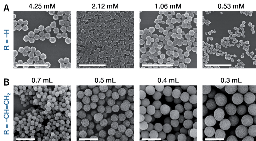
Fig. 36 SEM images of imine-linked COFs prepared in \text{CH}_3\text{CN} at room temperature. (A) TAPB-PDA COF with particle sizes of 200, 260, 290, and 330 nm prepared at varying aryl(triamine) monomer concentrations. Scale bar: 2 \mu\text{m} . Adapted with permission. 219 Copyright 2019, The Royal Society of Chemistry. (B) TAPB-DVA COF with particle sizes of 450, 800, 1000, and 1300 nm synthesized at different volumes of acetic acid. Scale bar: 2 \mu\text{m} . Adapted with permission. 222 Copyright 2019, American Chemical Society.
