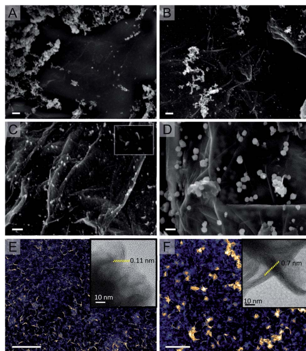
Fig. 1 (A–D) SEM images of \text{MoS}_2(1-x)\text{Se}_{2x}/\text{N-rGO} prepared using 6 \mu\text{l} of DMDSe: (A) ATM precursor – 15 h at 200 ^\circ\text{C} without step-temperature heating; (B) ATM – 10 h at 180 ^\circ\text{C} + 5 h 200 ^\circ\text{C} ; (C) ATM – 15 h at 180 ^\circ\text{C} + 5 h 200 ^\circ\text{C} (inset: detail of \text{MoS}_2(1-x)\text{Se}_{2x} slab); (D) \text{MoCl}_5 as Mo source – 15 h at 180 ^\circ\text{C} + 5 h 200 ^\circ\text{C} . (E and F) TEM of the sample shown in panel (C), before (E) and after annealing at 600 ^\circ\text{C} (F) (scale bar: 200 nm).
