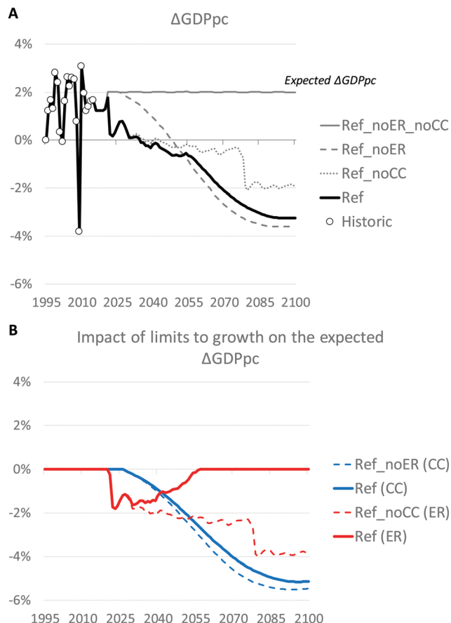
Fig. 10 Annual GDPpc variation and impact of limits to growth for each scenario case (1995–2100). (A) Achieved annual GDPpc growth rate ( \Delta GDPpc) for each scenario case. (B) Impact of limits to growth on the expected annual GDPpc growth ( \Delta GDPpc) due to energy scarcity (red lines, ER) and climate change damages (blue lines, CC).
