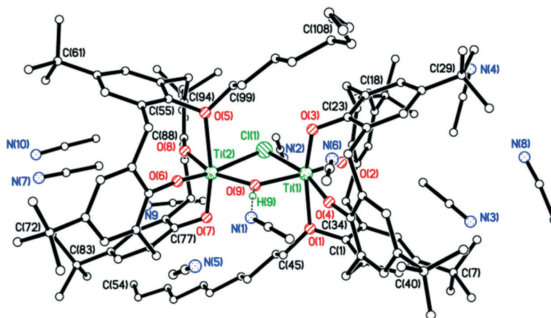
Fig. 7 Molecular structure of \{[\text{TiL}(\text{O})_3(\text{On-decyl})]_2(\mu\text{-Cl})(\mu\text{-OH})\} \cdot 8.5\text{MeCN} ( 10 \cdot 8.5\text{MeCN} ) (most H atoms are omitted for clarity). Selected bond lengths (Å) and angles ( ^\circ ): Ti(1)–O(1) 2.381(3), Ti(1)–O(2) 1.817(3), Ti(1)–O(3) 1.852(3), Ti(1)–O(4) 1.793(3), Ti(1)–O(9) 2.000(3), Ti(1)–Cl(1) 2.5177(14); O(1)–Ti(1)–O(3) 168.54(13), O(2)–Ti(1)–O(4) 102.84(15), Cl(1)–Ti(1)–O(9) 74.82(10), Ti(1)–O(1)–C(1) 112.8(2), Ti(1)–O(2)–C(12) 150.5(3), Ti(1)–O(3)–C(23) 119.9(2), Ti(1)–O(4)–C(34) 168.3(3).
