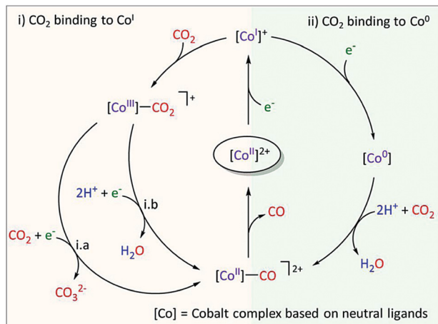
Fig. 8 Proposed mechanism of \text{CO}_2 reduction with Co27 . During CPE at the \text{Co}^{\text{III/I}} wave, trace amounts of CO were released. A formal oxidation state is given for the different Co species. Reprinted with permission from ref. 41. Copyright (2020) American Chemical Society.
