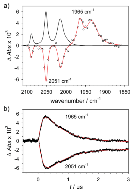
Fig. 5 (a) Transient IR spectrum 0.3 \mu\text{s} after excitation (O, \color{red}{\text{---}} ) and normalized IR spectrum of the starting state ( \text{---} ) for formation of \mathbf{1H} by reduction of \mathbf{1H}^+ (obtained by protonation of \mathbf{1} with 2.6 mM \text{Cl}_2\text{BSA} ) with flash-quench generated [\text{Ru}(\text{dmb})_3]^+ in acetonitrile. (b) Kinetic traces ( \cdots ) and fits ( \color{red}{\text{---}} ) monitoring pseudo-first order formation of \mathbf{1H} ( 1965\text{ cm}^{-1} ) and bleach of \mathbf{1H}^+ ( 2051\text{ cm}^{-1} ) followed by pseudo-first order decay of \mathbf{1H} by protonation with \text{Cl}_2\text{BSA} and charge recombination with \text{TTF}^+ .
