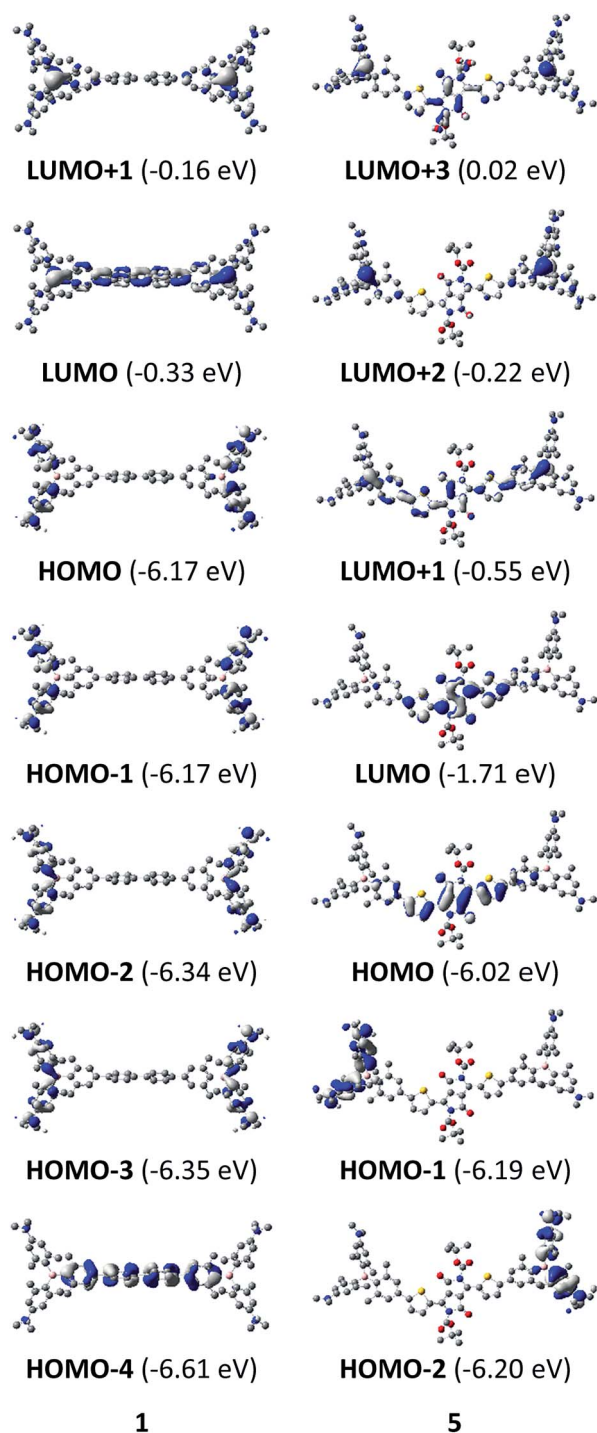
Fig. 2 DFT (CAM-B3LYP/6-31G(d))-calculated relevant orbitals for 1 and 5 . Hydrogen atoms are omitted for clarity. Surface isovalue: \pm 0.03 [ a_0^{-3/2} ]. Orbital energy differences are not direct approximations of excitation energies. They are provided here for comparison between the compounds.
