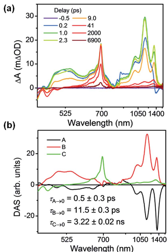
Fig. 4 (a) fsTA spectra and (b) decay-associated spectra (DAS) of Per \subset TTzExVBox 4+ in CH 3 CN excited at 414 nm ((A) formation of Per 2+ –TTz 2+ , (B) decay of Per 2+ –TTz 2+ , (C) decay of unbound 1 *Per). The wavelength axis is plotted in reciprocal space. Time constants are for the representative data set shown here; averages and standard deviations from multiple experiments are given in Table 1.
