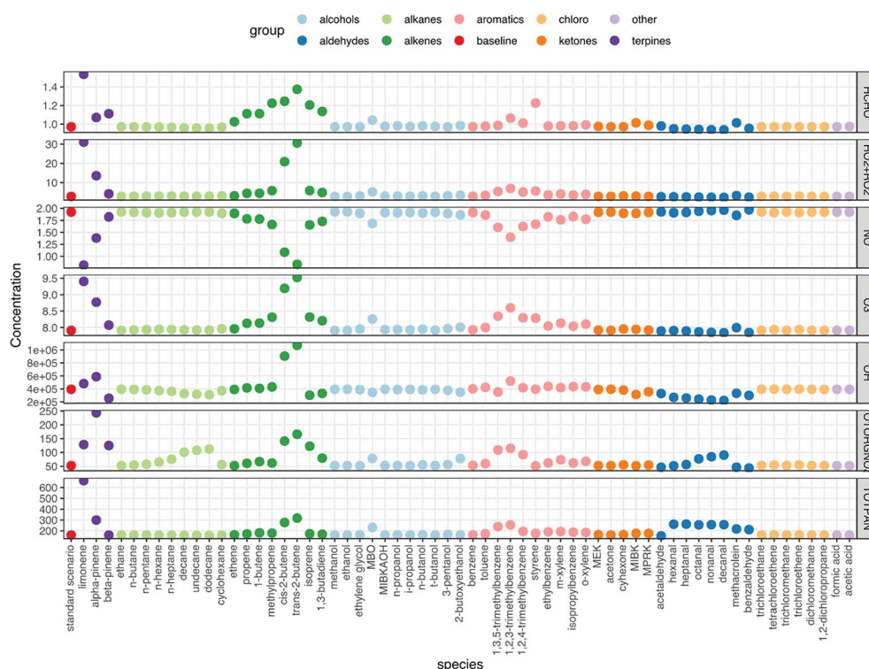
Fig. 2 Changes in mixing ratio for HCHO (ppb), \Sigma\text{HO}_2 + \text{RO}_2 (ppt), NO (ppb), O 3 (ppb), \Sigma organic nitrate species (ppt) and \Sigma PAN species (ppt) and concentration of OH (molecule per cm 3 ), with the addition of 10 ppb of different VOCs in turn. The molecules are colour coded according to functionality (see legend) and the standard run (with no VOCs added indoors) is shown in red.
