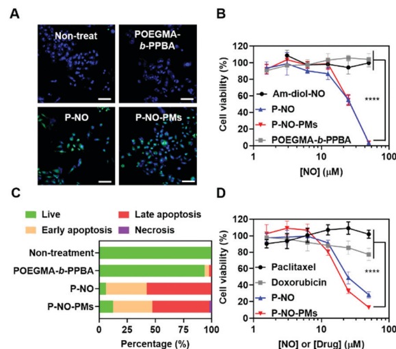
Fig. 3 In vitro behavior of P-NO-PMs. (A) Intracellular NO release of P-NO-PMs. Nuclei and intracellular NO were stained with DAPI (blue) and DAF-2-DA (green). Scale bar is 100 \mu\text{m} . (B) Anticancer effects and (C) live/dead assay in MCF-7. (D) Anticancer effects in MCF-7/ADR cell lines.
